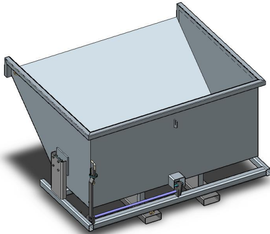
(Type ROB18 standard model shown) Refer 'ROB_WL_Sales' Product Specification sheet for Wheels & Crane Lug options.
